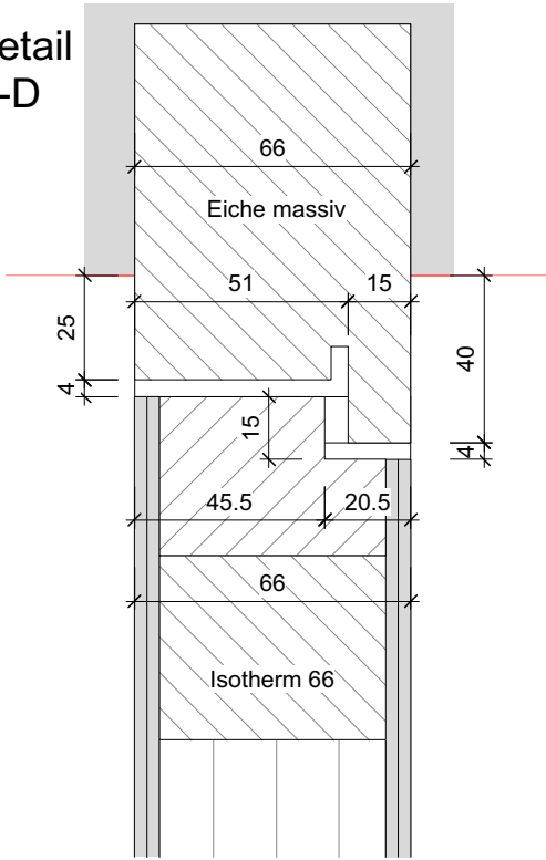
Detail D-D
